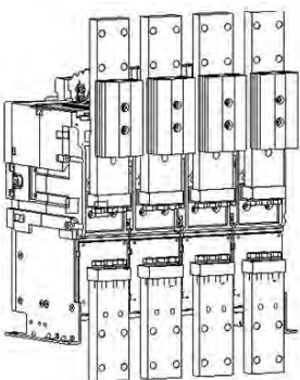
Front Flat Terminations
