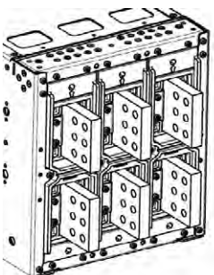
Envelope 1 and 2, 3 Pole 1600A
