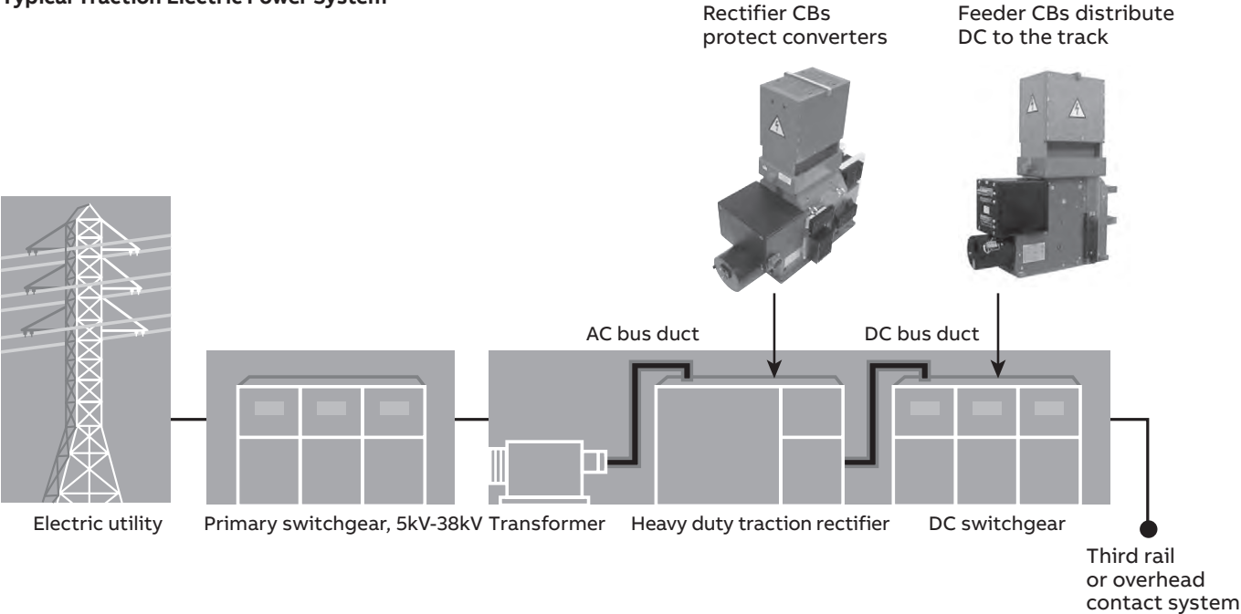
Typical Traction Electric Power System
